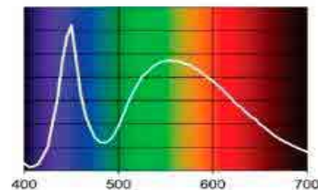
Spectral Power Distribution Standard White LED with CRI 70 (Ra)
